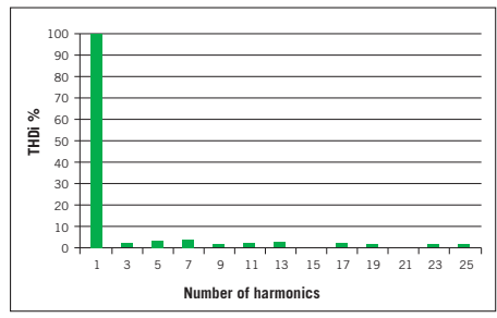
Typical measurement with FINHRM5
