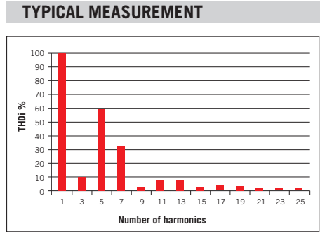
Typical measurement without FINHRM5
